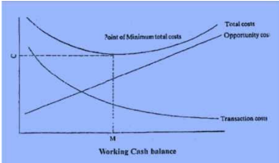
Figure 1.4: The Optimal Working Cash Balance
