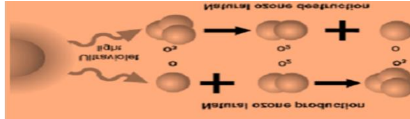
Fig: 2.2: ozone production and destruction cycle
